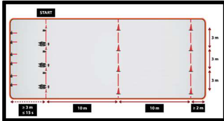
Figure 3.1: Example of an acceptable FORCE circuit test set-up.
